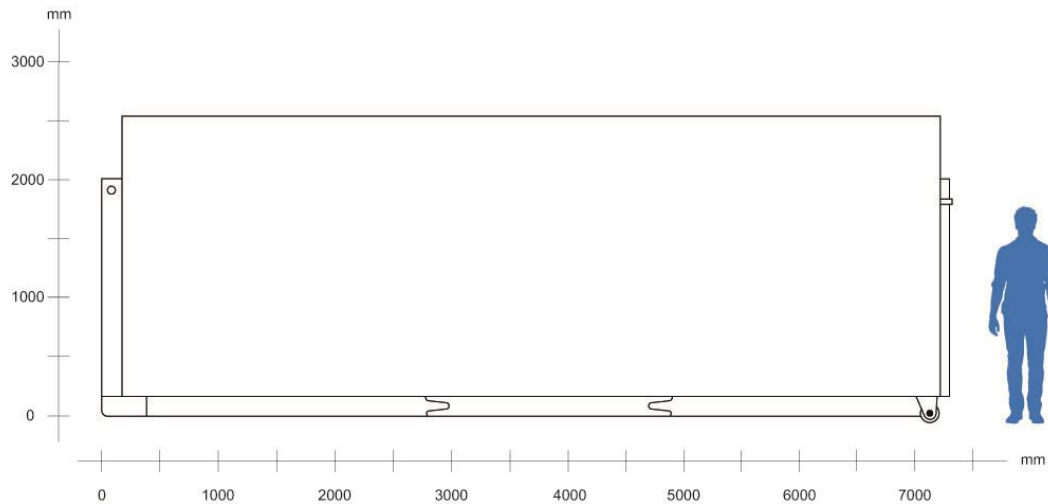
Gleitabrollcontainer (GAK) Inhalt ca. 43,0 m 3 ca. 7,35m x 2,70m x 2,50m (L x H x B)
